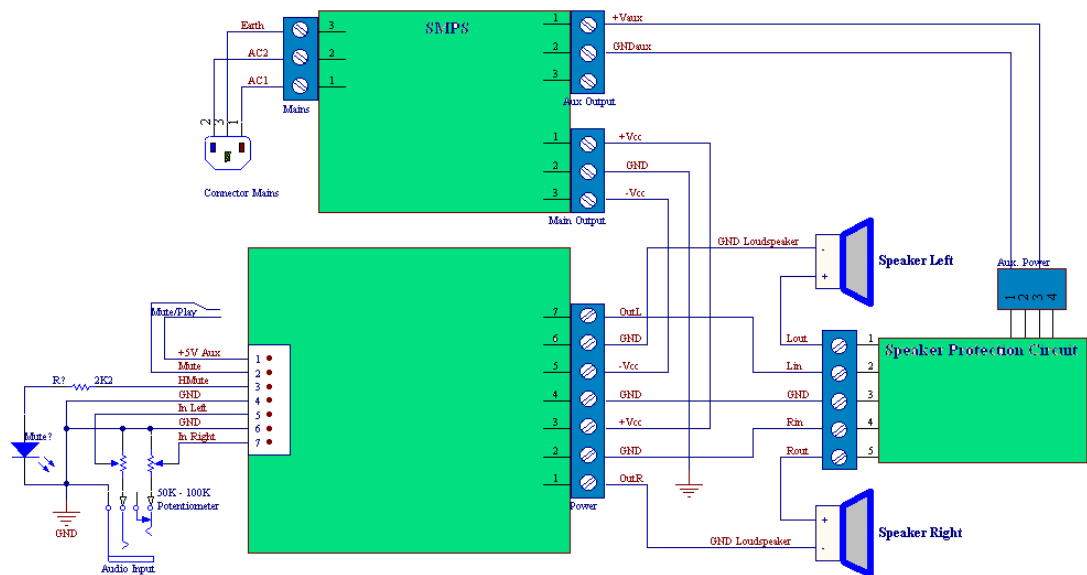
Figure 7: TA3020v3b Amplifier Connection Diagram using SMPS and Speaker Protection Circuit board.
