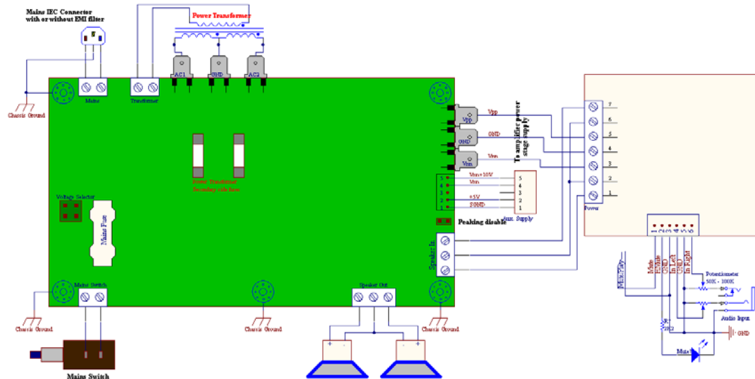
Figure 6: TA3020v3b Amplifier Connection Diagram using Power Supply and Protection Circuit board.
