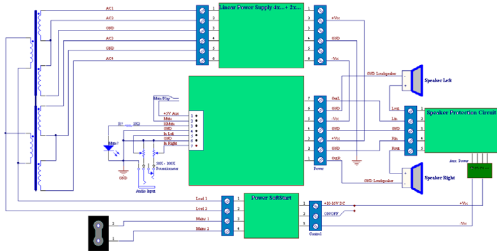
Figure 5: TA3020v3b Amplifier Basic Connection Diagram using PSS, Speaker Protection Circuit, Linear supply board.
