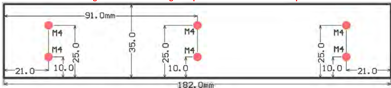
Fig.6 SMPS2000R heatslug size and drill pattern
