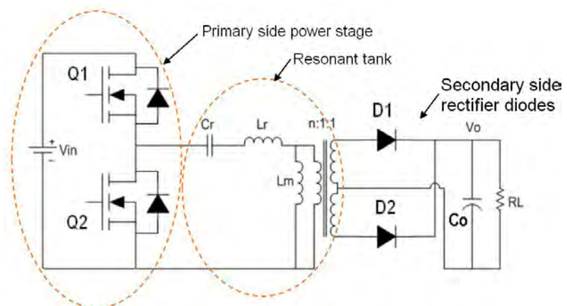
Fig.2 SMPS2000R simplified block diagram
