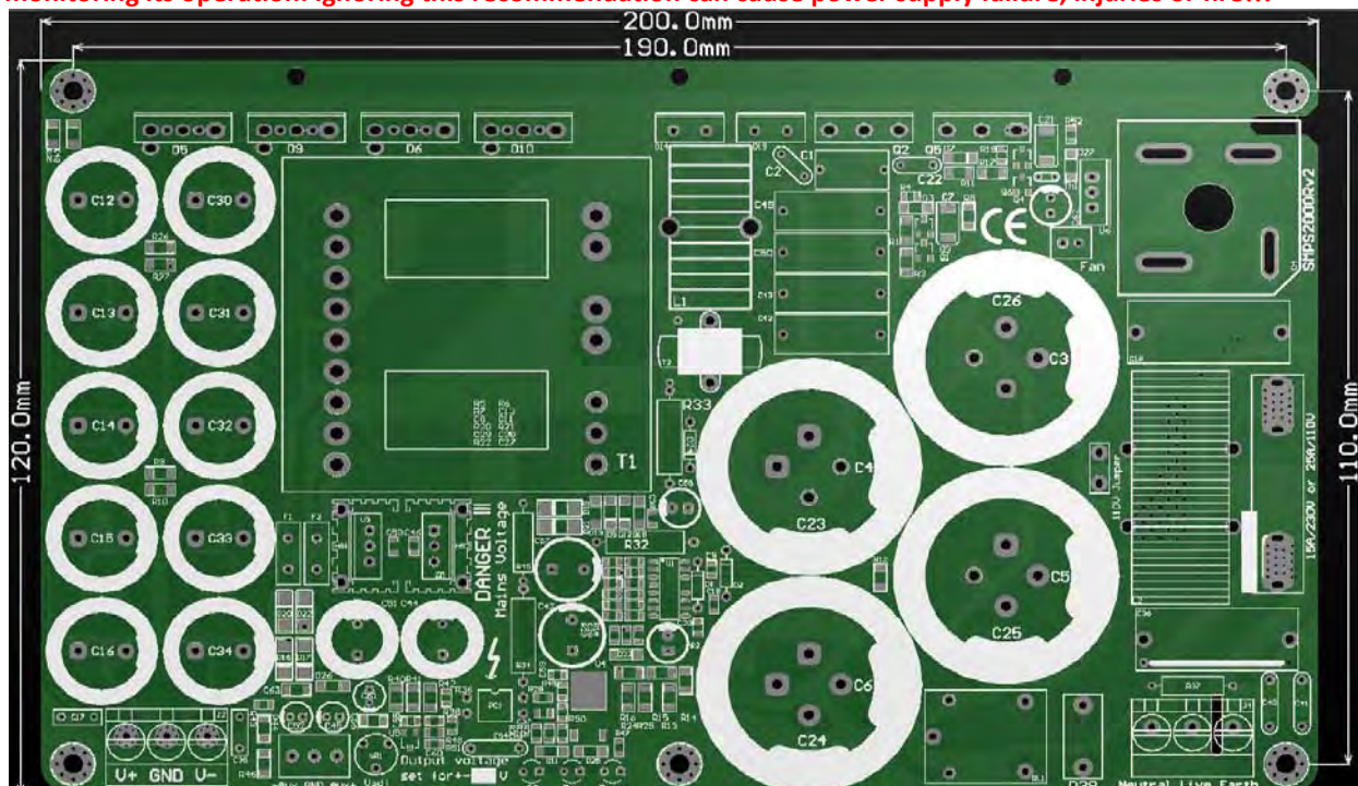
Fig.6 SMPS2000R PCB Board Layout and size
