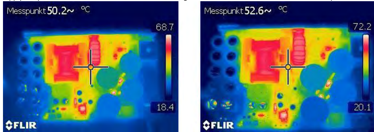
Fig.5 SMPS2000R thermal image after running 30min and 60min loaded with 2x800W class D amplifier as load
