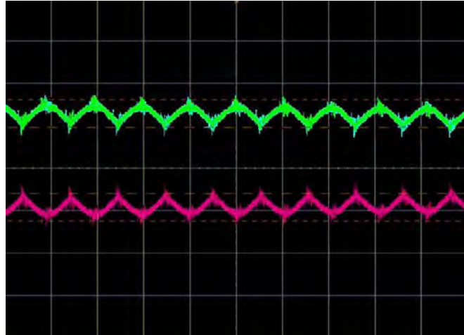
Fig.3 SMPS2000R output ripple ±84V output voltage version
